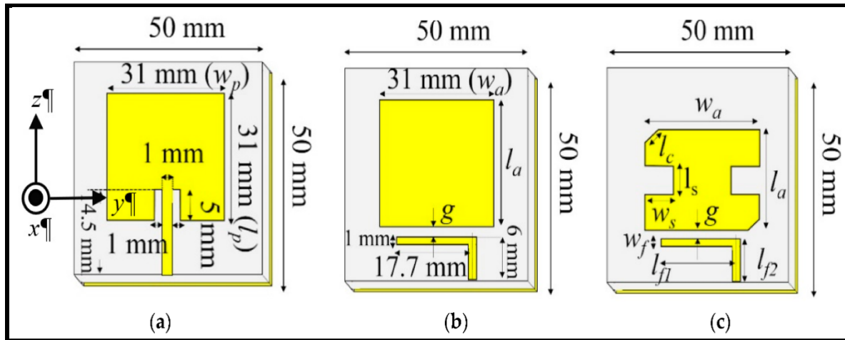
Fig 6 : Design methods of antenna
